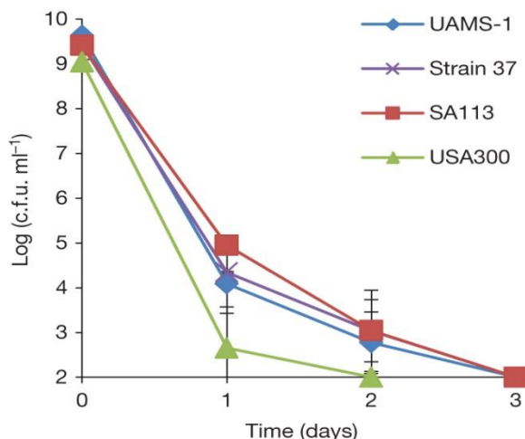
Figure 4. S. aureus was grown in MHB for 16 h and challenged with 10x MIC of ADEP4 and rifampicin. Colony counts were performed every 24 h. The x axis is the limit of detection. Data are representative of 3 independent experiments. Error bars represent standard deviation.
